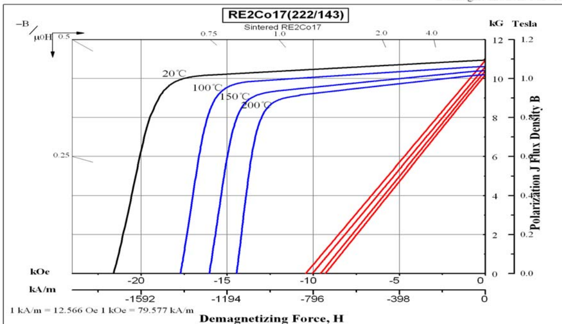
Demagnetization Curves
