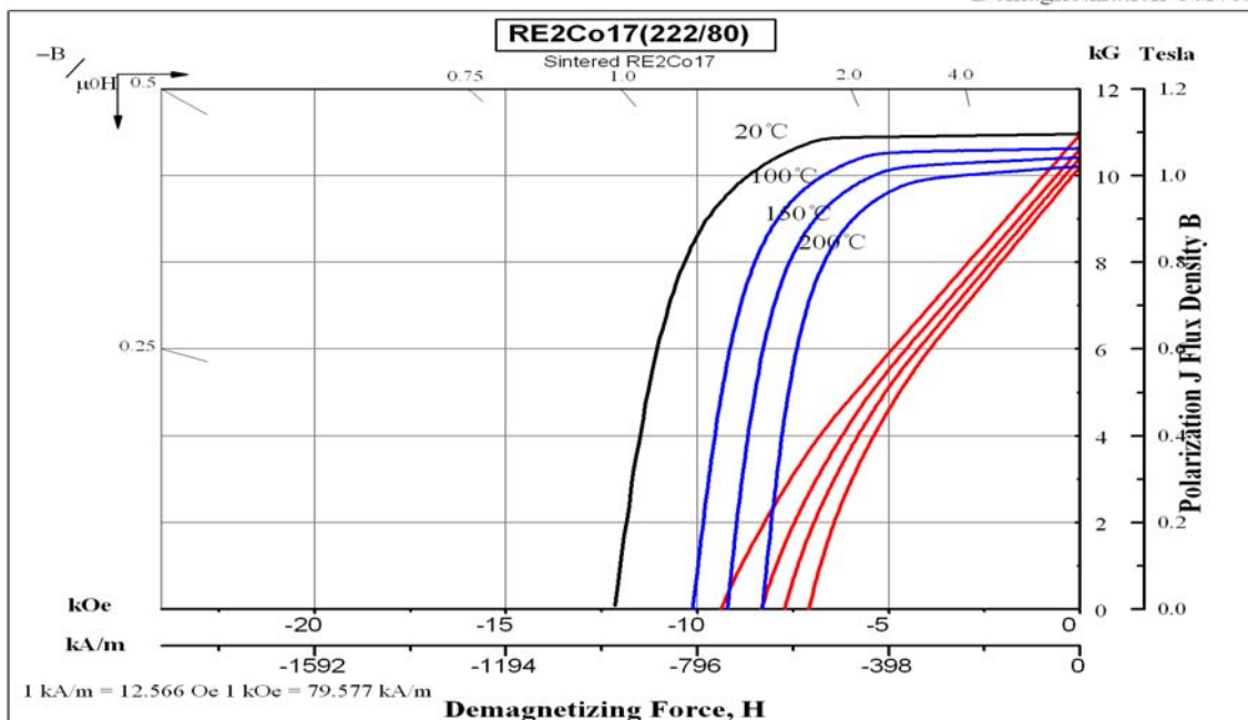
Demagnetization Curves
