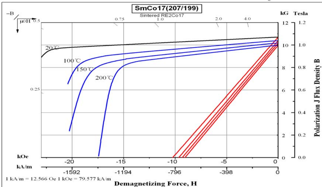
Demagnetization Curves
