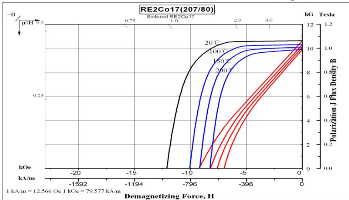
Demagnetization Curves
