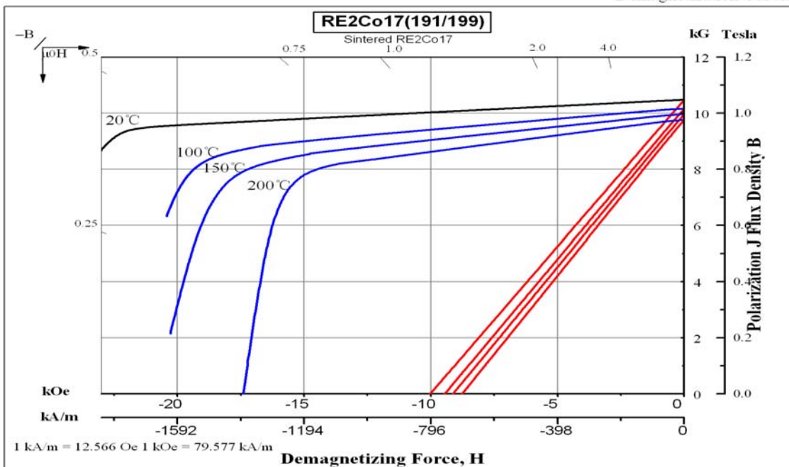
Demagnetization Curves
