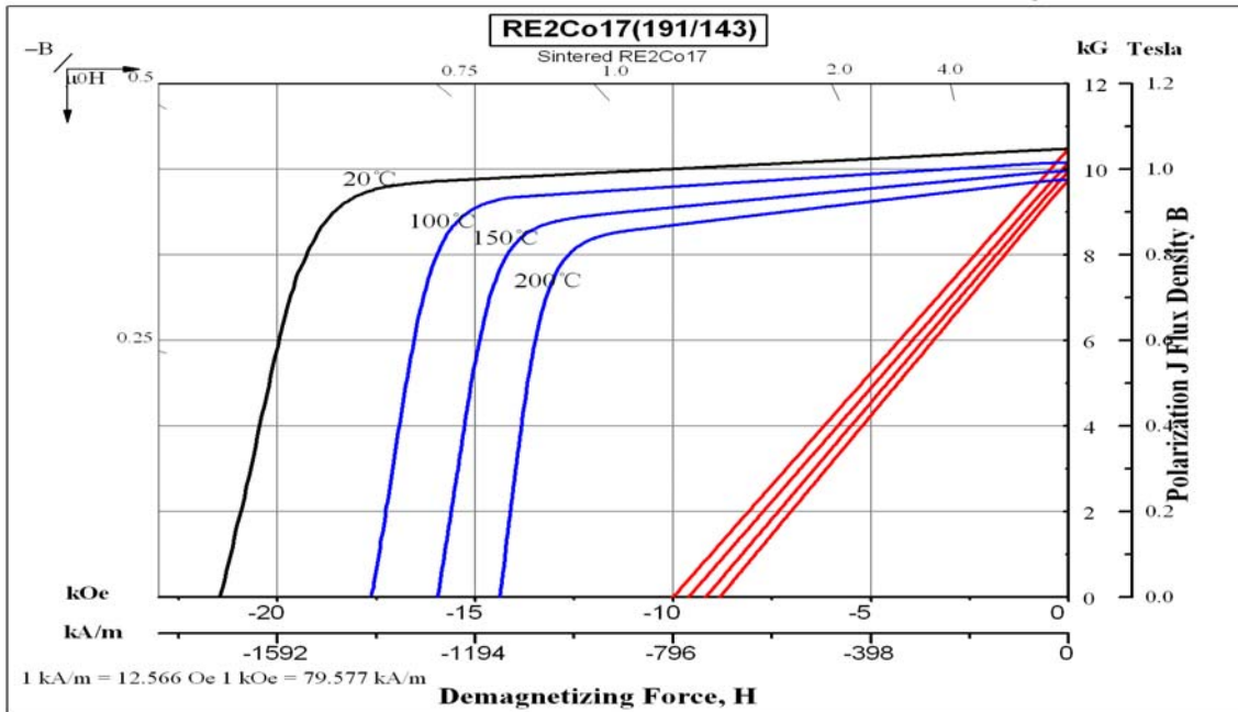
Demagnetization Curves
