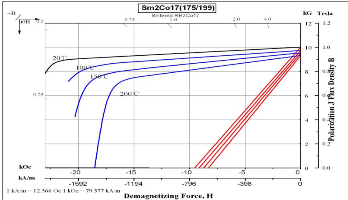
Demagnetization Curves
