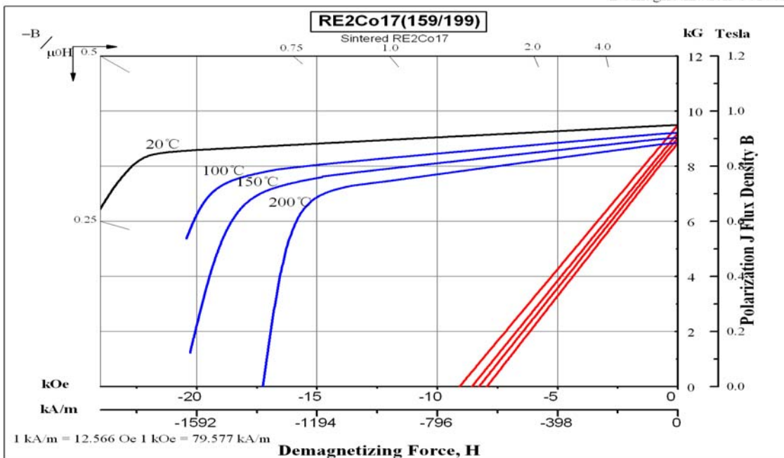
Demagnetization Curves
