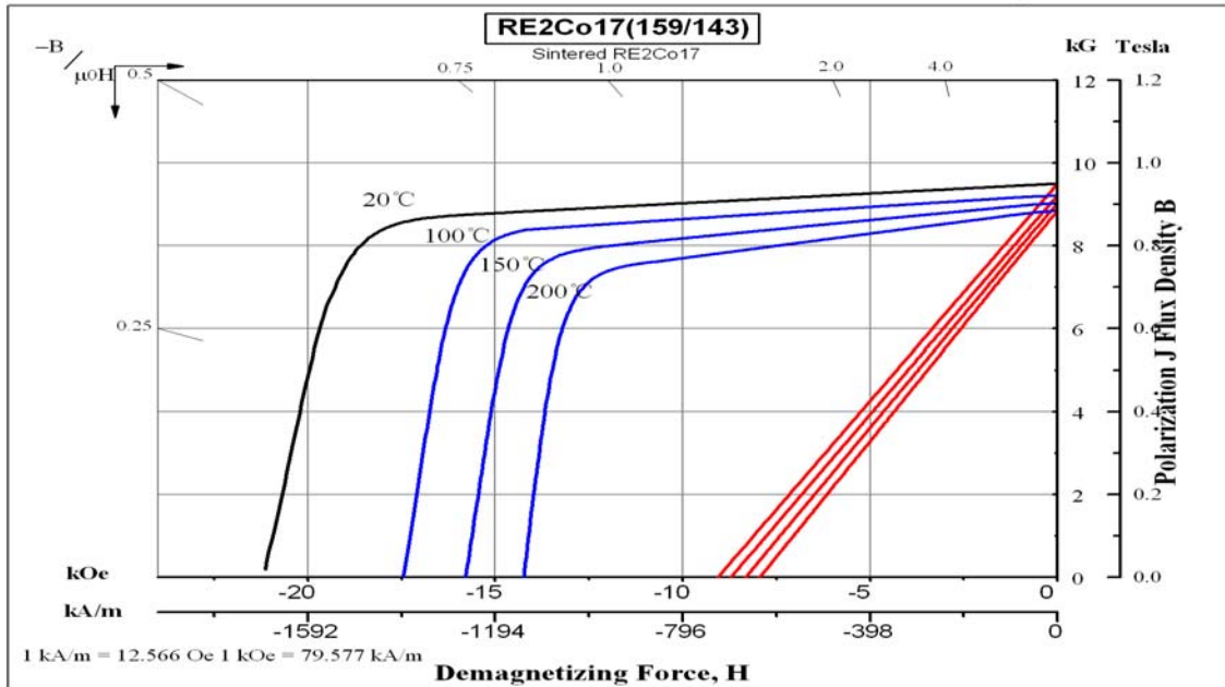
Demagnetization Curves
