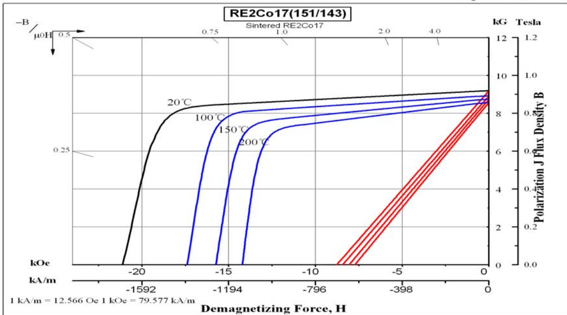
Demagnetization Curves
