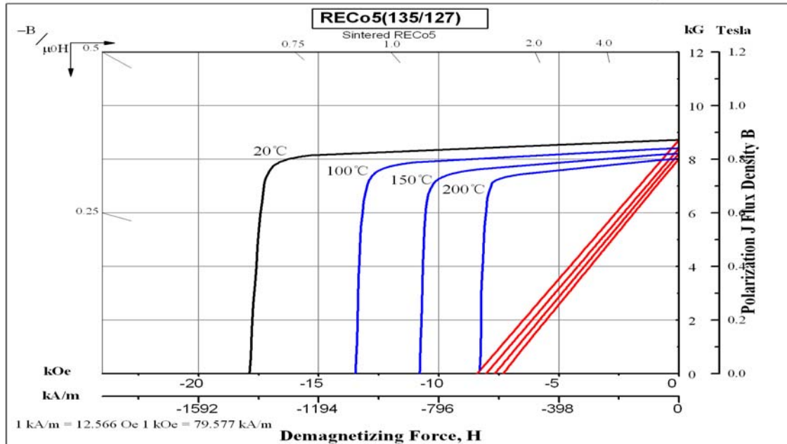
Demagnetization Curves
